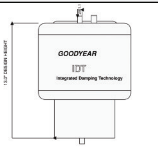
SIDE VIEW HEIGHT AND WIDTH
