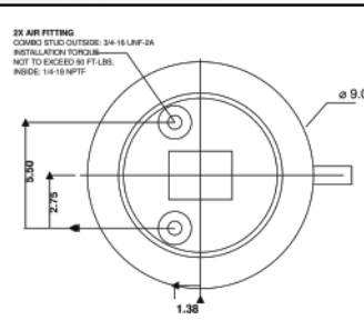
UPPER MOUNTING VIEW
